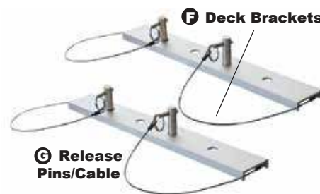
FIGURE 6 ) Attach Dock Ladder to the Deck Brackets, using Clevis Pins (E) and Release Pins (G).
