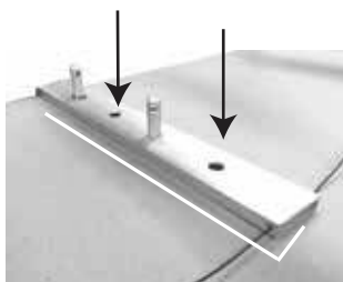
FIGURE 5 ) Attach Deck Brackets (F) to the wood deck with wood screws (not included).
