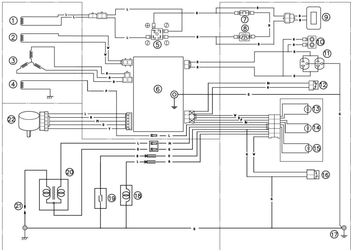
Wiring Diagram
