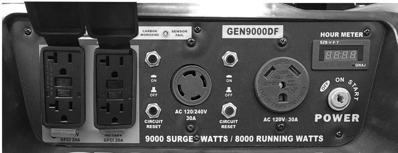
Figure 8 - Outlets available on this generator, from left to right: 4 each 120V GFCI AC , 120/240V AC, 120V AC RV.
